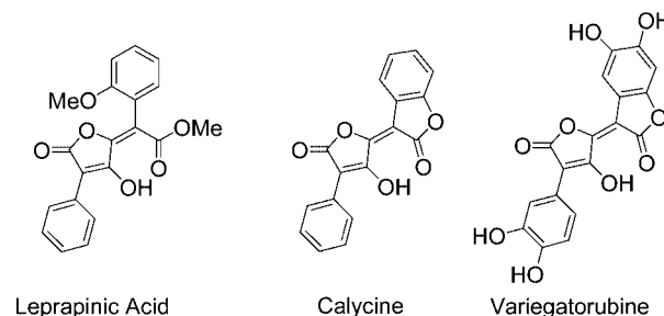
Scheme 1. Leprapinic acid, calycine and variegatorubine.
